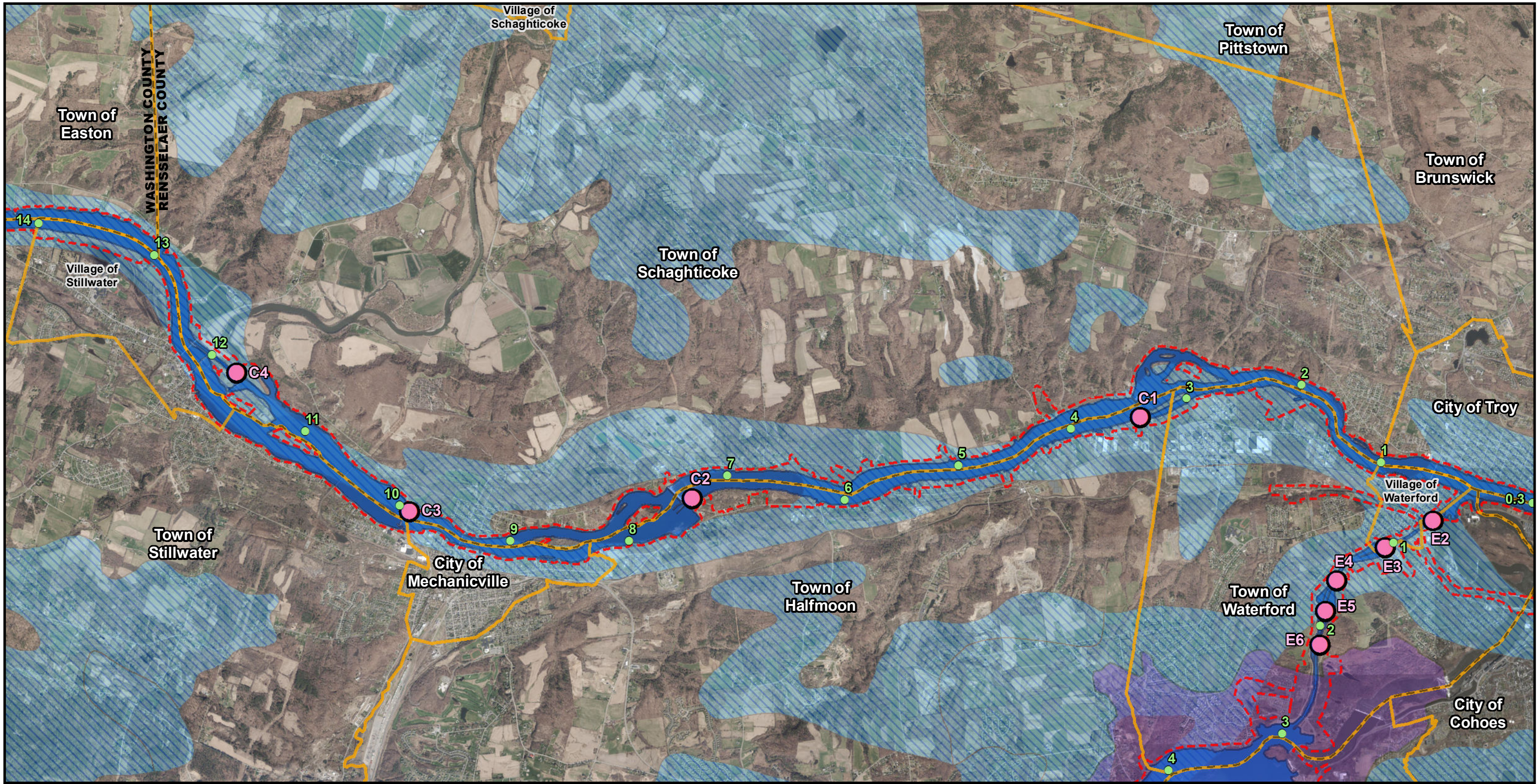
Figure 14F: Aquifers
